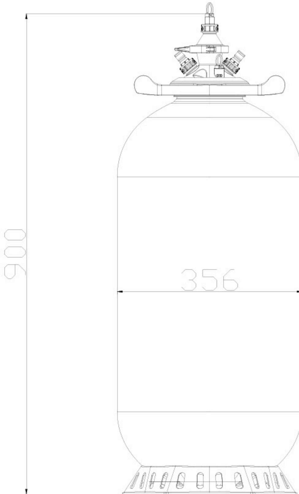
60L All Rounder Mega Grip Dimensions - Tri Clover Lid
