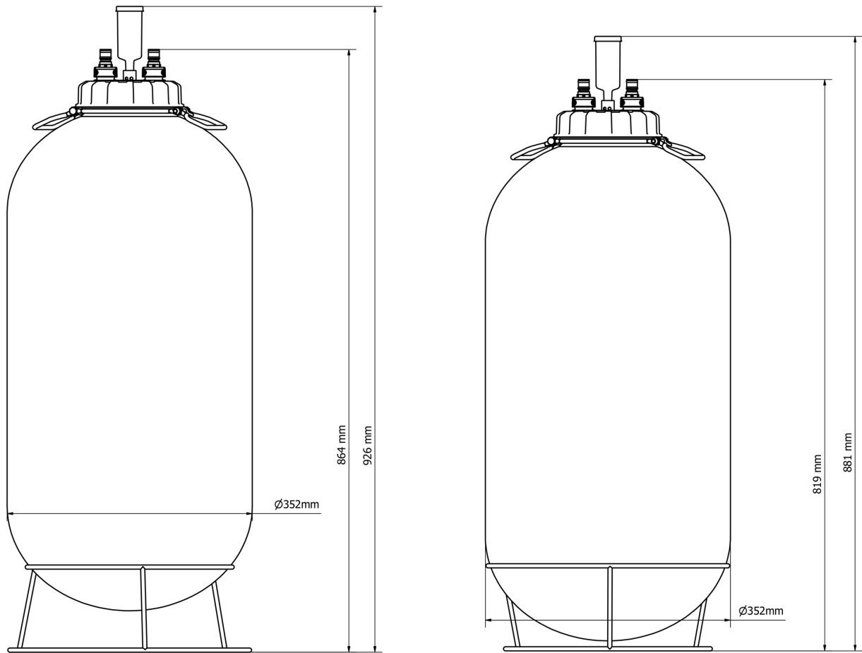
60L All Rounder | Dimensions
