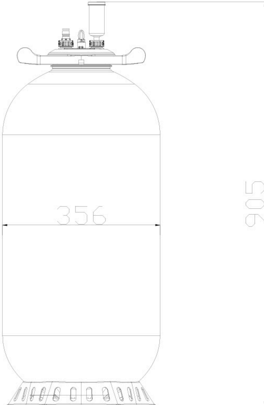
60L All Rounder Mega Grip Dimensions
