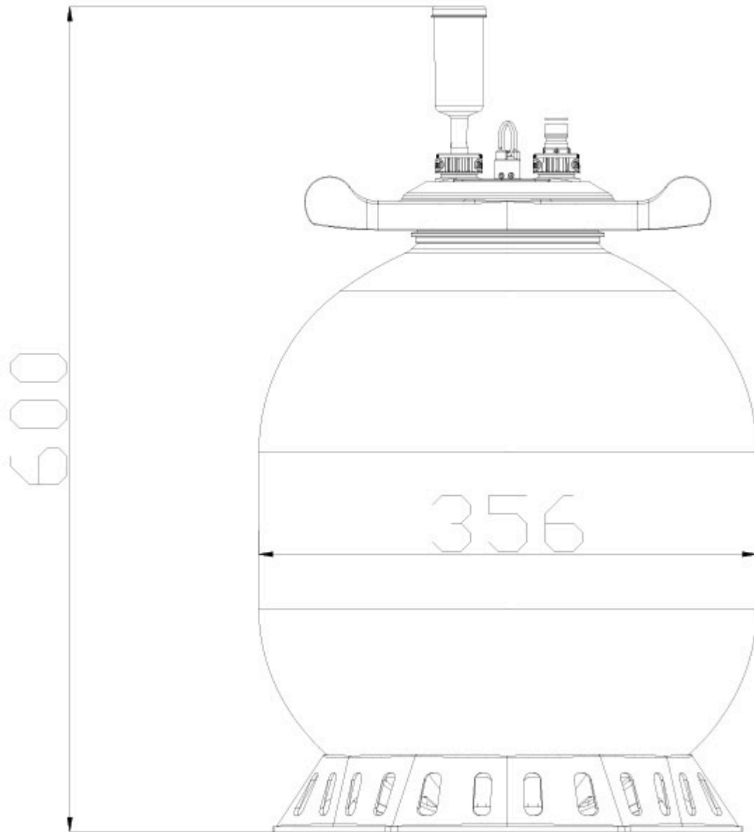
30L All Rounder Mega Grip Dimensions
